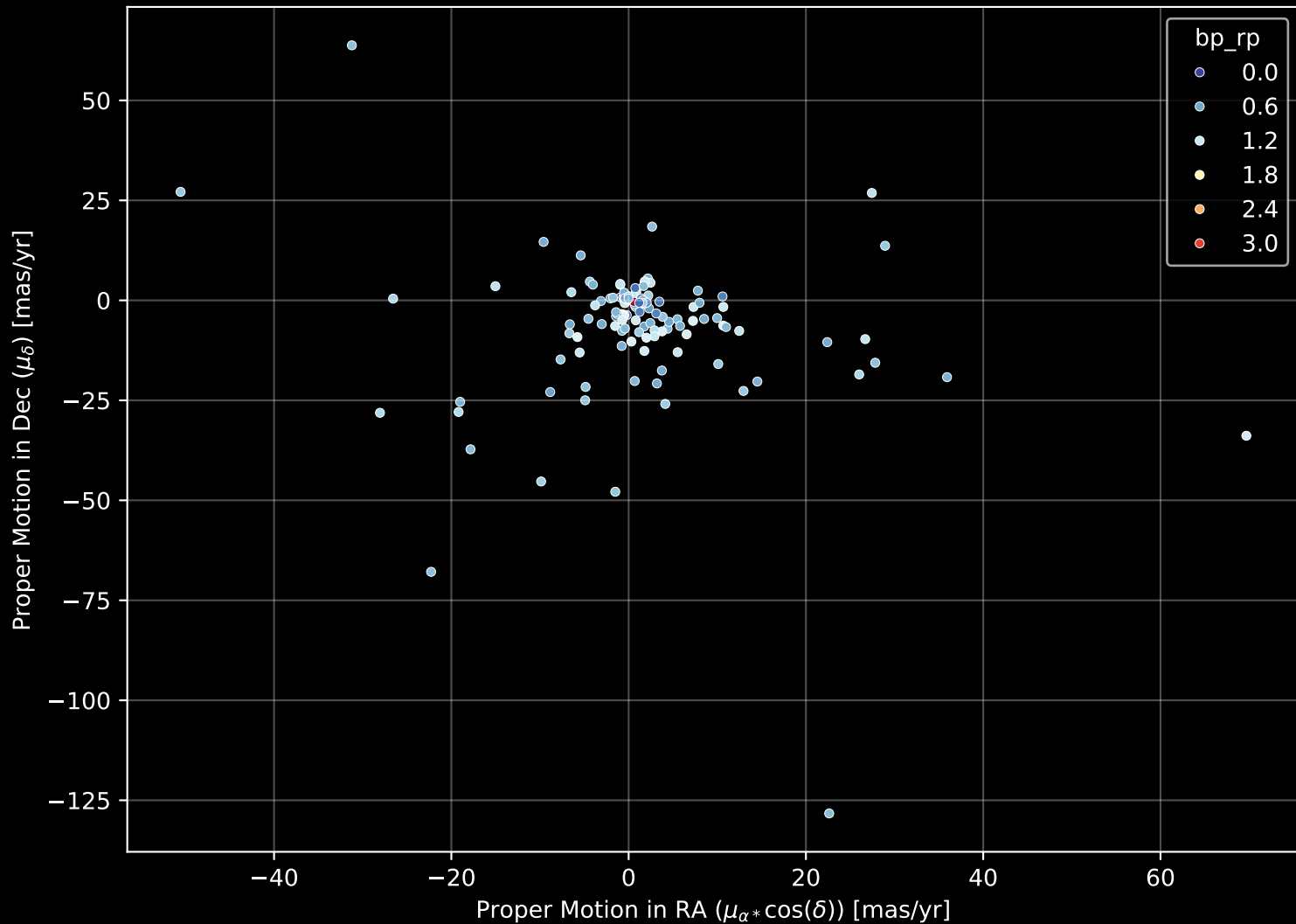
GALAH DR4 Field: [2545] Proper Motion Diagram (n= 139)
