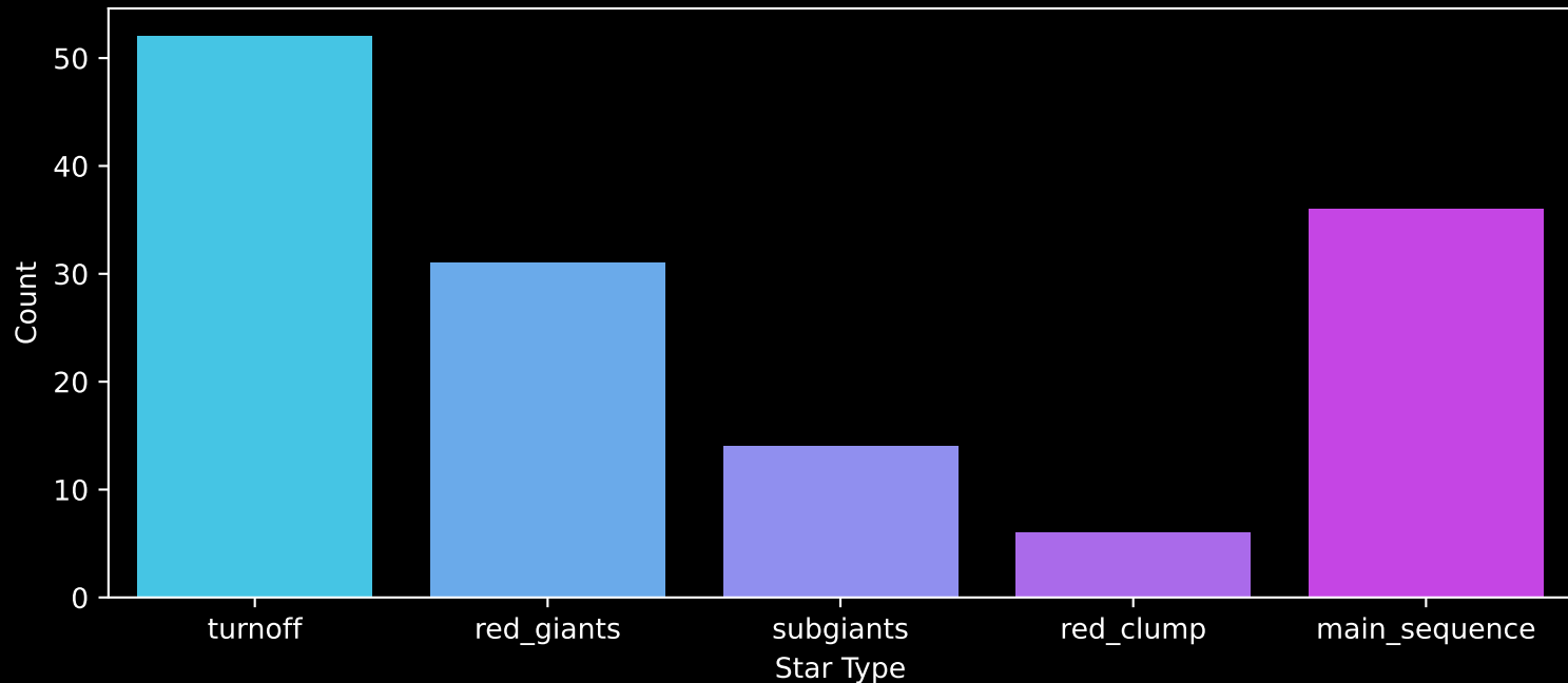
GALAH DR4 Field: [2545] Count plot of Star Type
