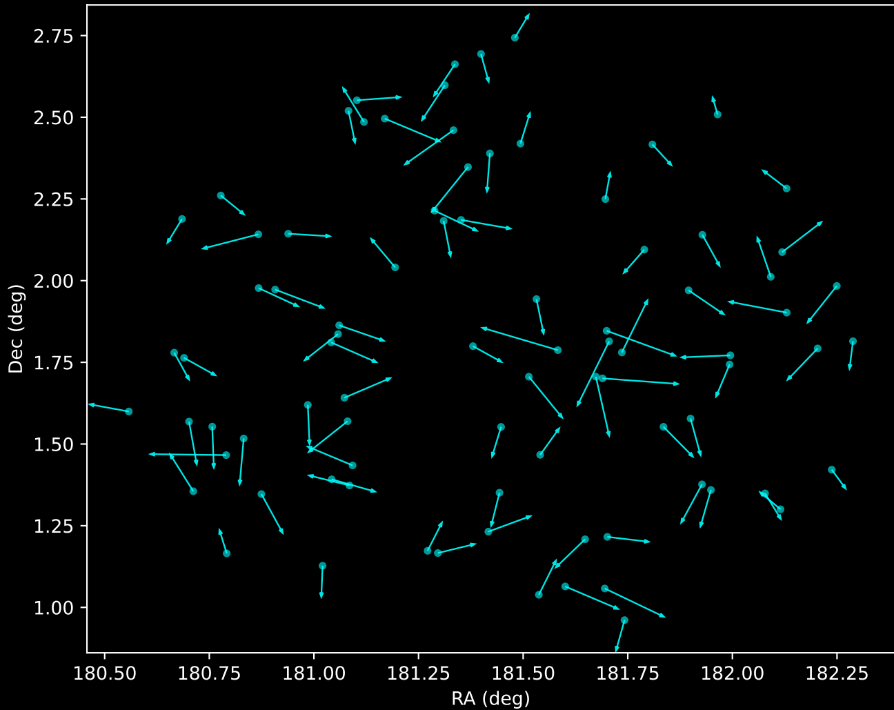
GALAH DR4 Noise Stream Proper Motion Vectors (n=85)
