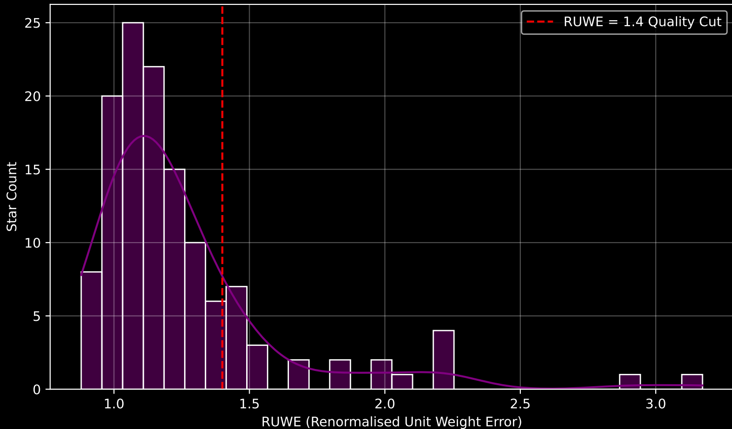
GALAH DR4 Field [2545] RUWE Distribution (n= 129)
