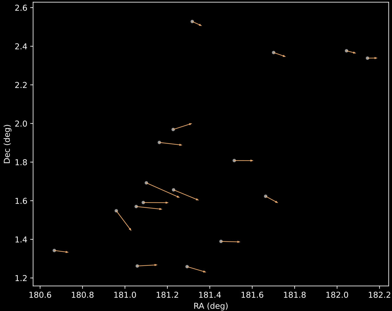
GALAH DR4 Cluster 3 Proper Motion Vectors (n=17)
